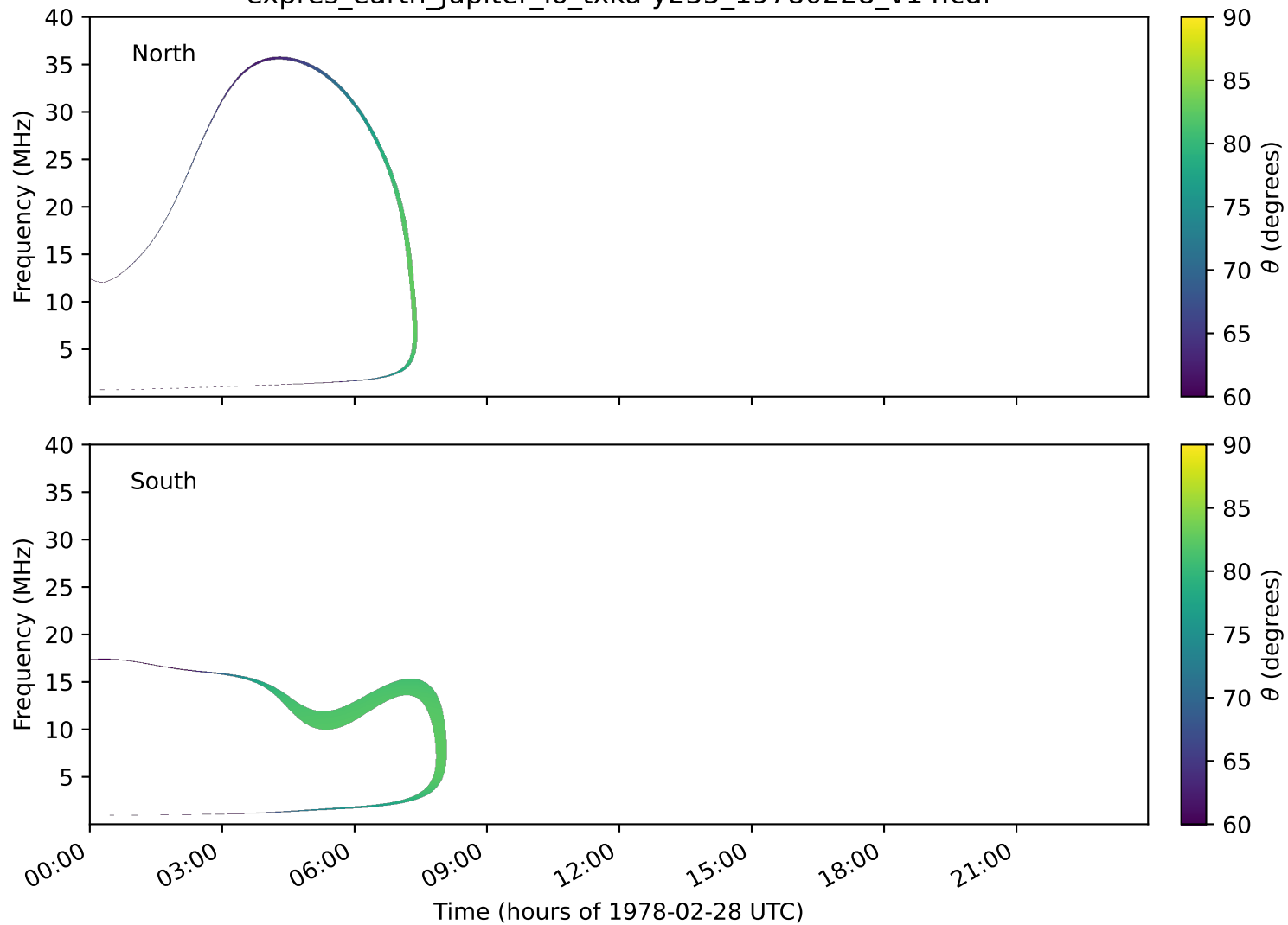
expres_earth_jupiter_io_txka-y235_19780228_v14.cdf
