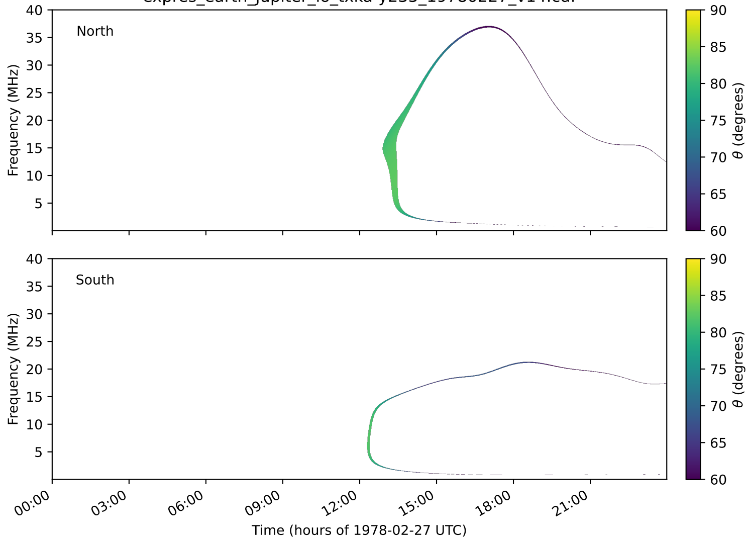
expres_earth_jupiter_io_txka-y235_19780227_v14.cdf
