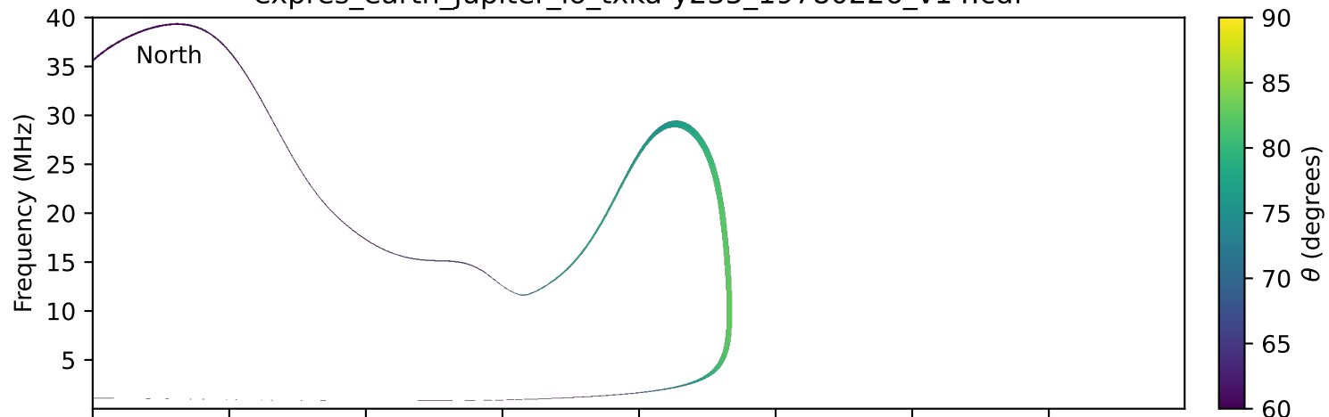
expres_earth_jupiter_io_txka-y235_19780226_v14.cdf
