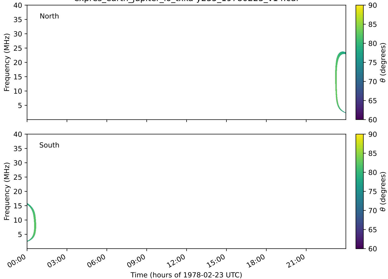
expres_earth_jupiter_io_txka-y235_19780223_v14.cdf
