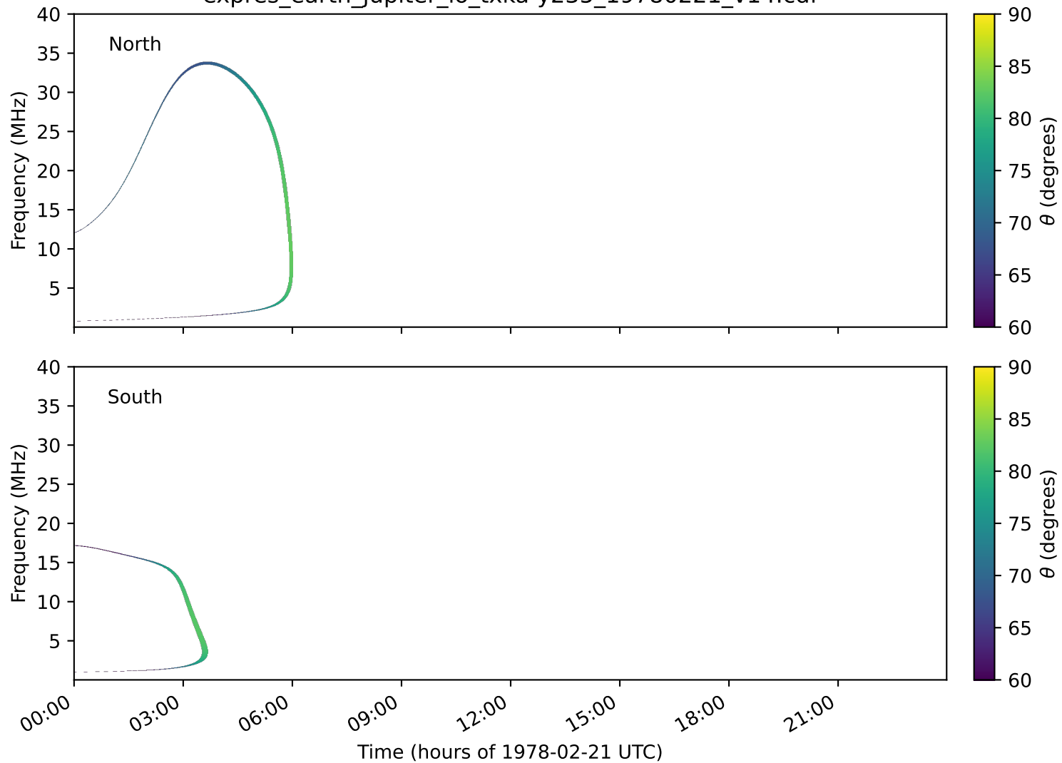
expres_earth_jupiter_io_txka-y235_19780221_v14.cdf
