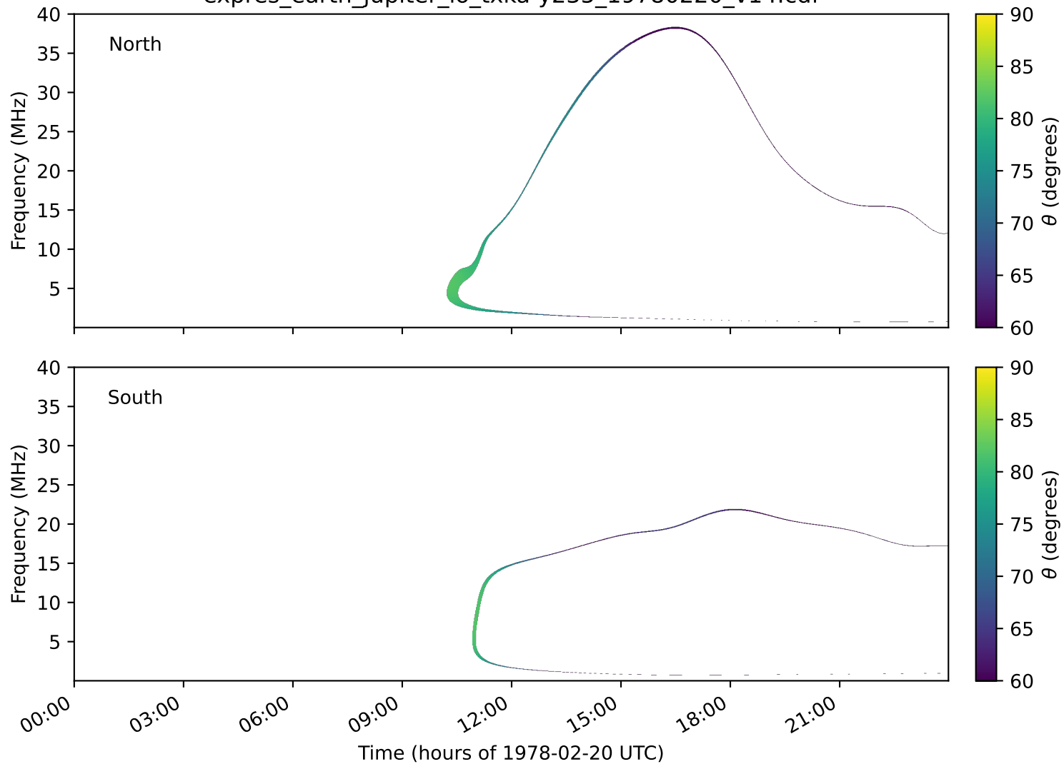
expres_earth_jupiter_io_txka-y235_19780220_v14.cdf
