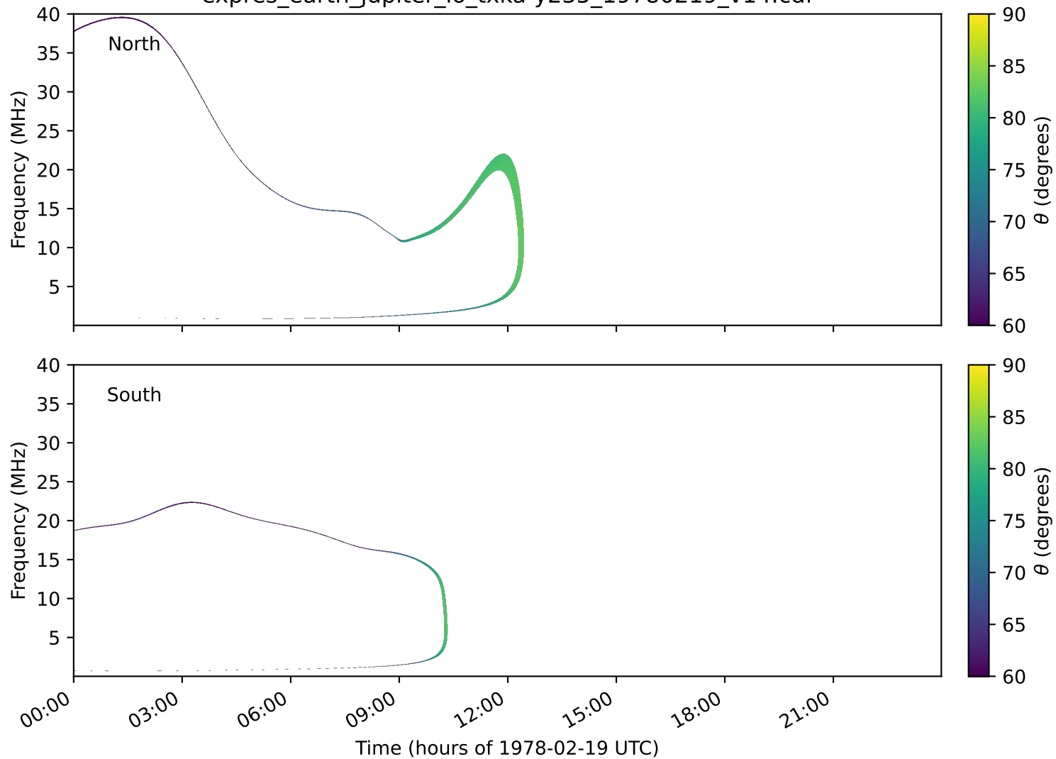
expres_earth_jupiter_io_txka-y235_19780219_v14.cdf
