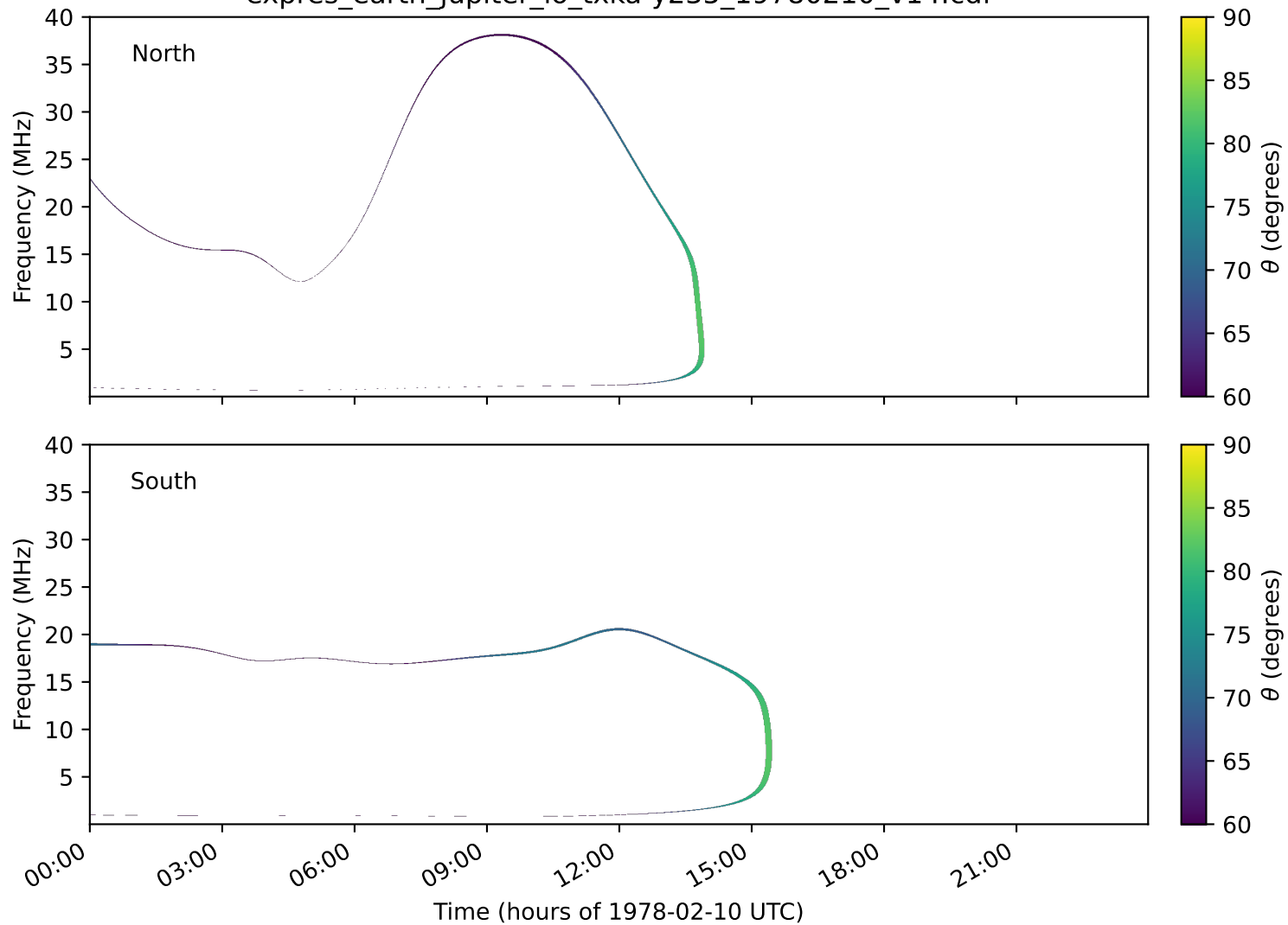
expres_earth_jupiter_io_txka-y235_19780210_v14.cdf
