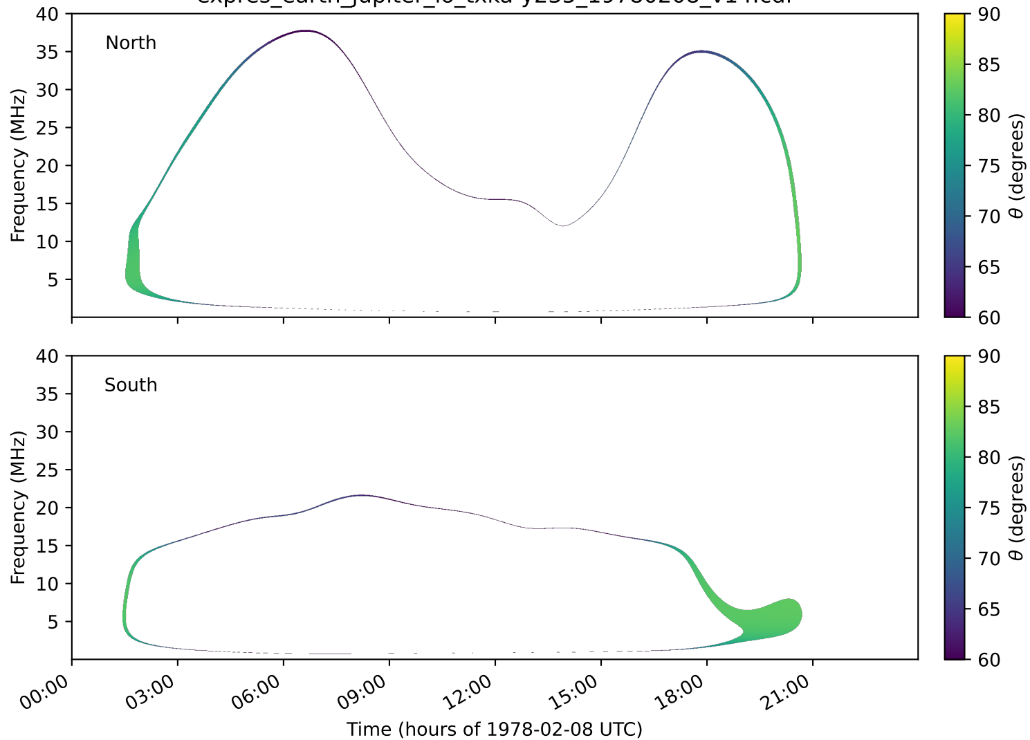
expres_earth_jupiter_io_txka-y235_19780208_v14.cdf
