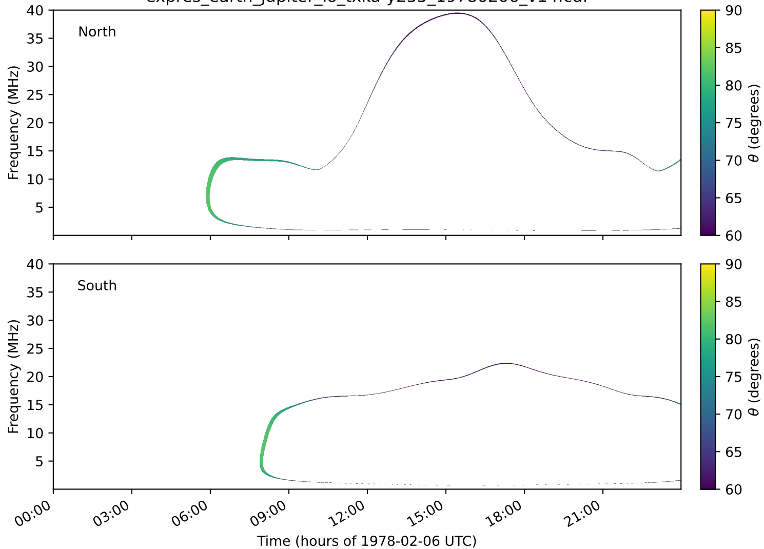
expres_earth_jupiter_io_txka-y235_19780206_v14.cdf
