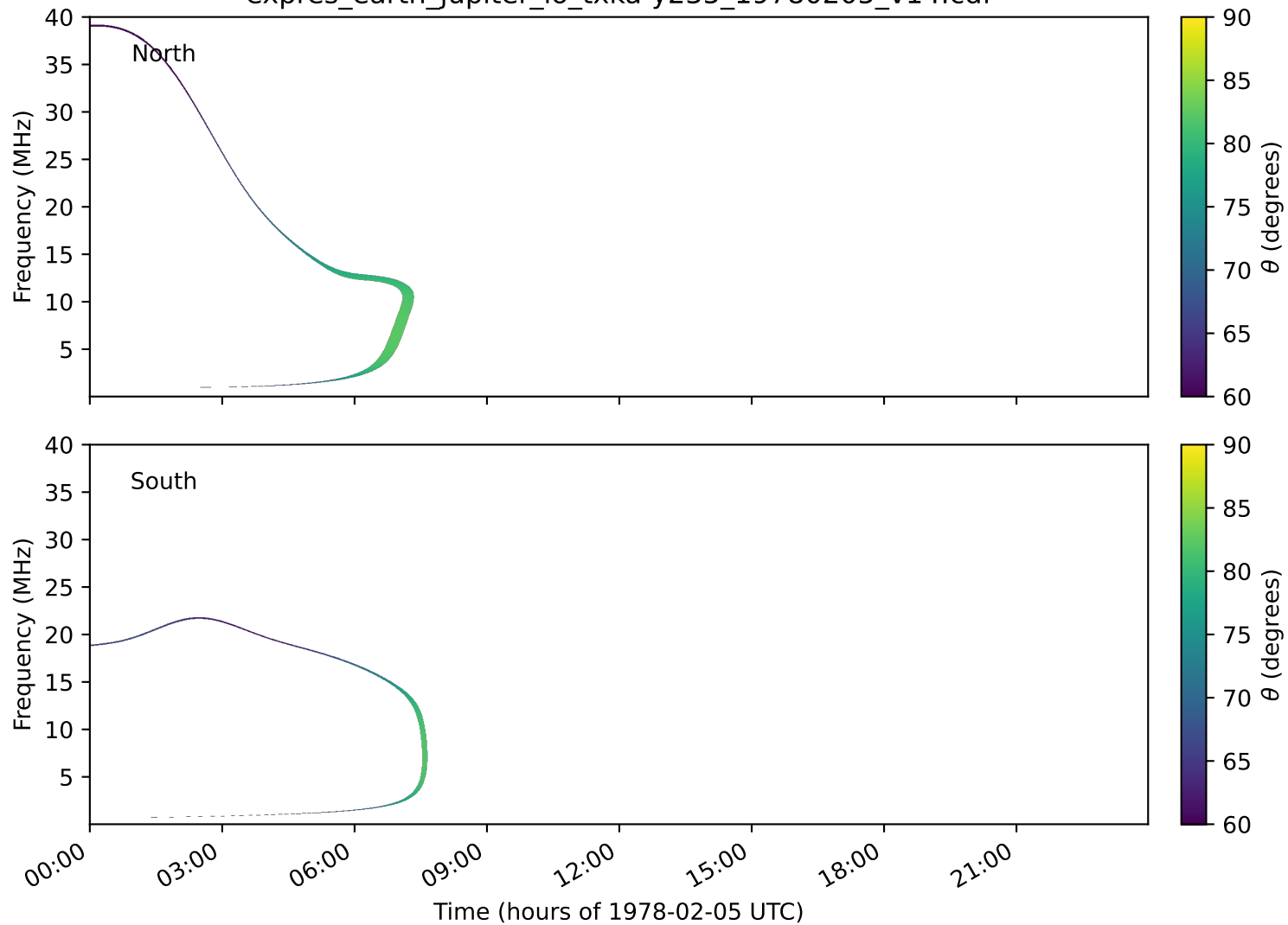
expres_earth_jupiter_io_txka-y235_19780205_v14.cdf
