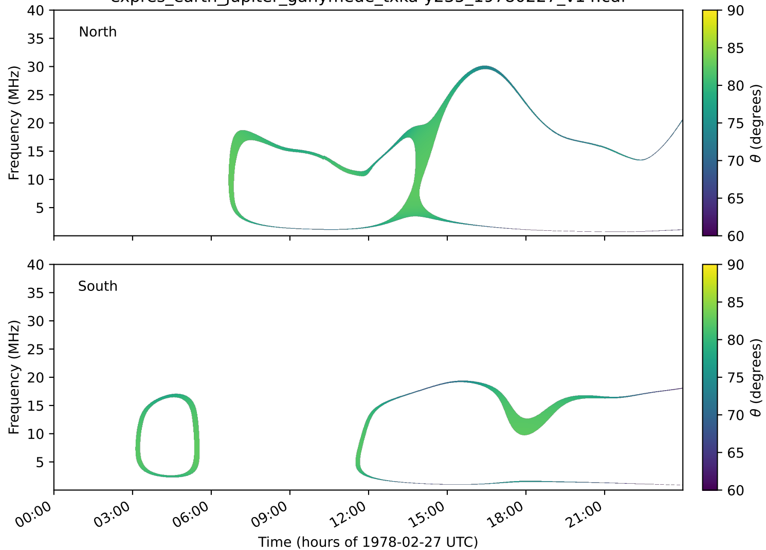
expres_earth_jupiter_ganymede_txka-y235_19780227_v14.cdf
