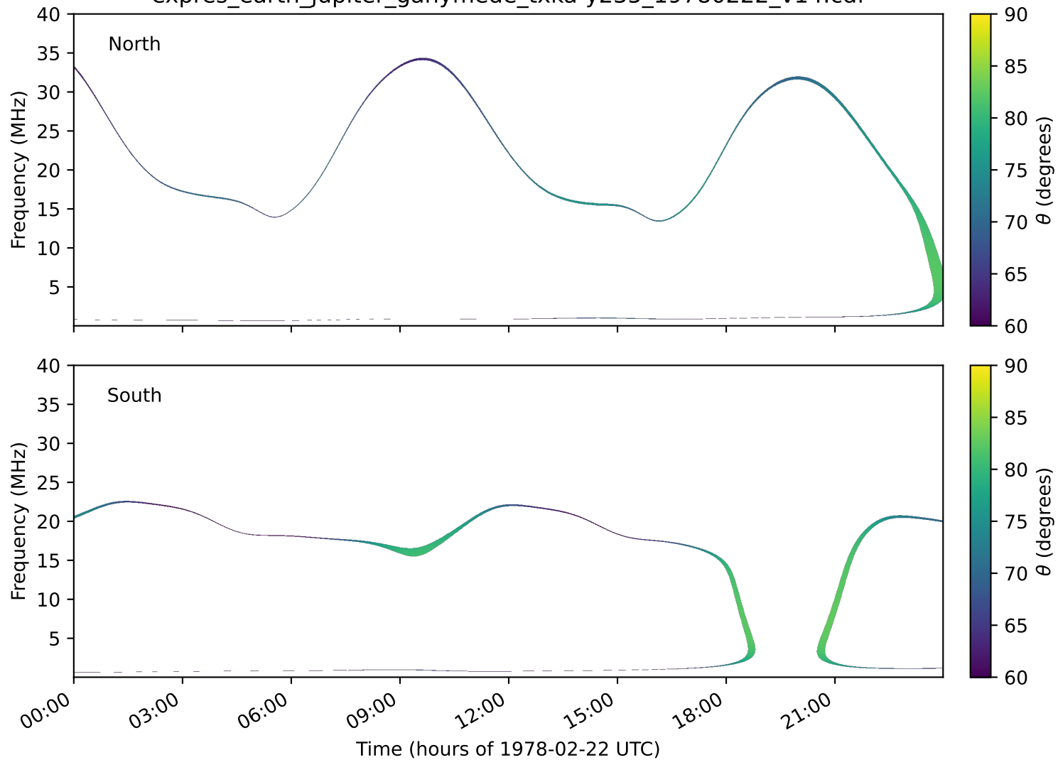
expres_earth_jupiter_ganymede_txka-y235_19780222_v14.cdf
