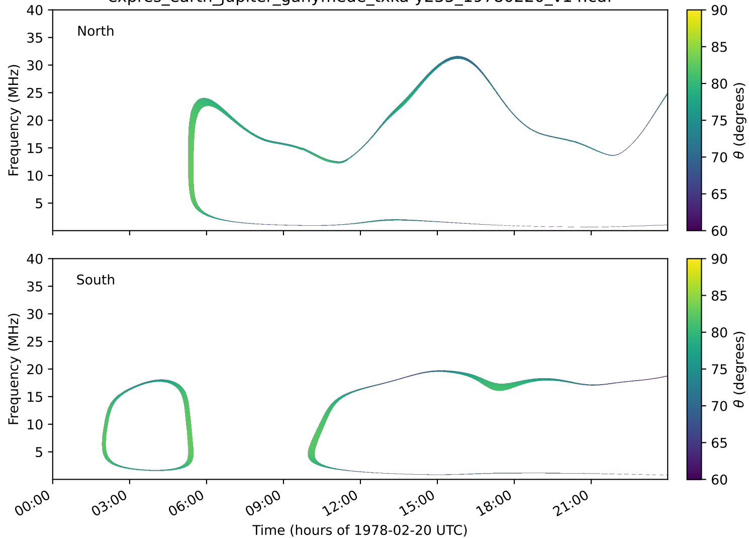
expres_earth_jupiter_ganymede_txka-y235_19780220_v14.cdf
