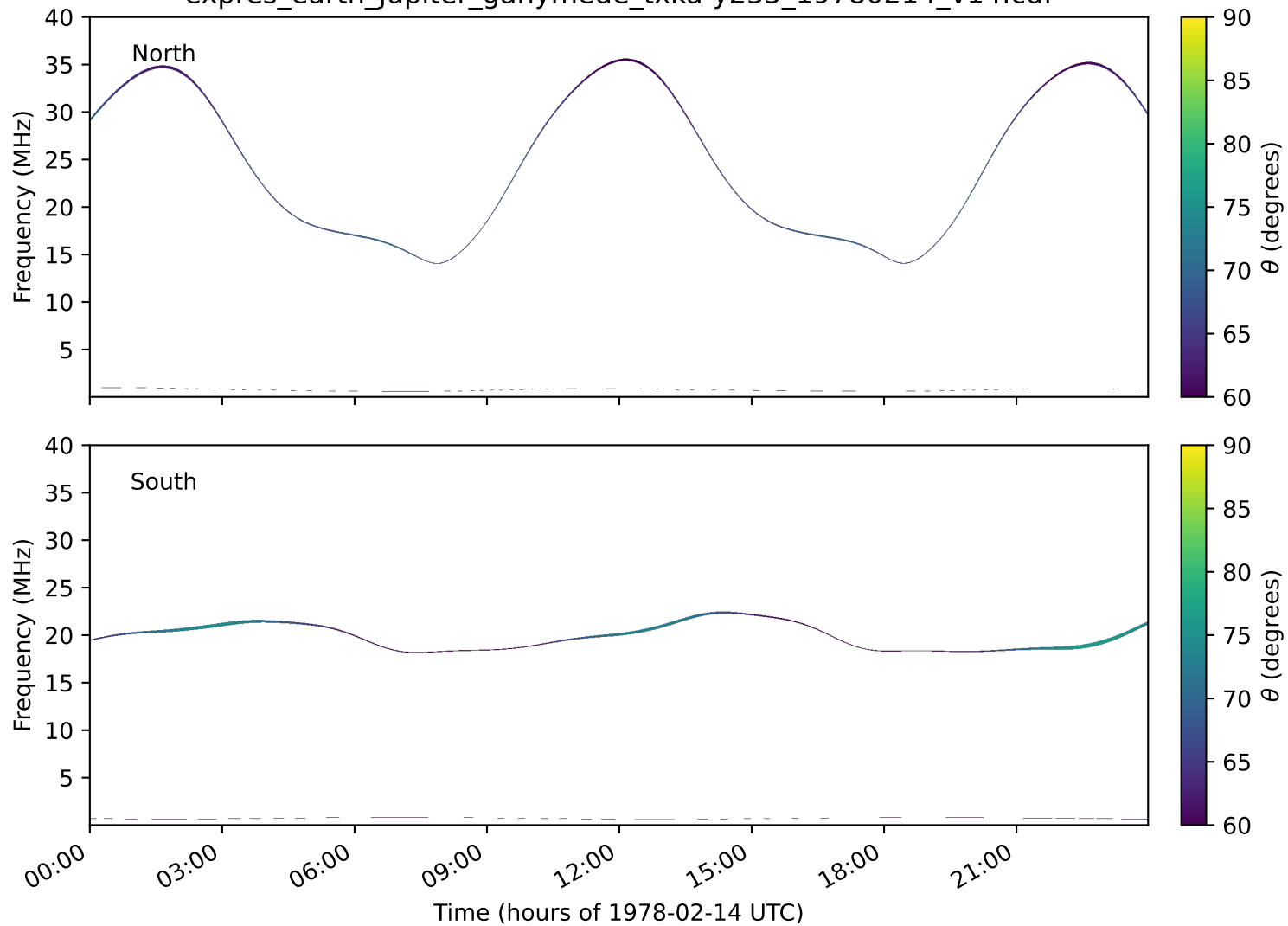
expres_earth_jupiter_ganymede_txka-y235_19780214_v14.cdf
