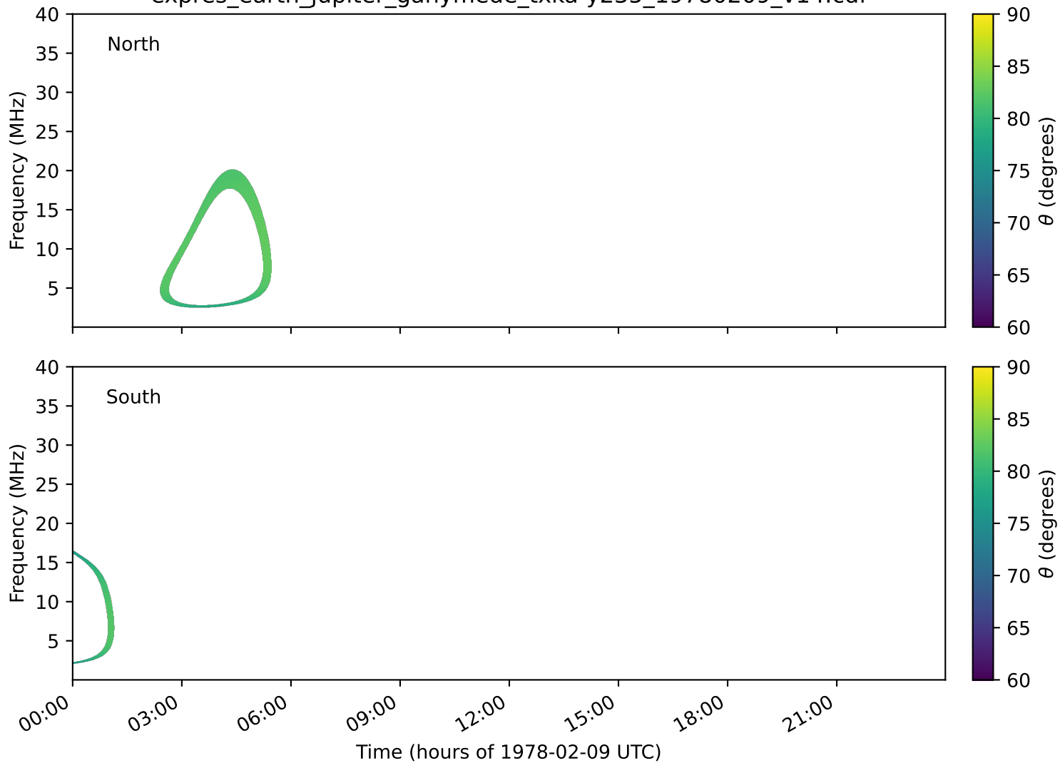
expres_earth_jupiter_ganymede_txka-y235_19780209_v14.cdf
