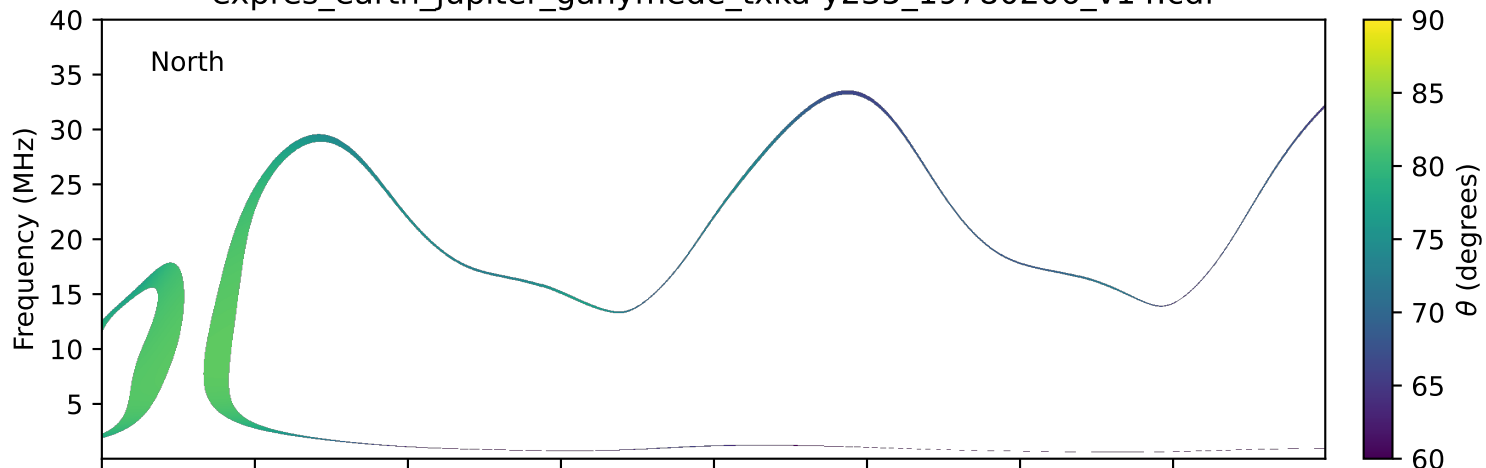
expres_earth_jupiter_ganymede_txka-y235_19780206_v14.cdf
