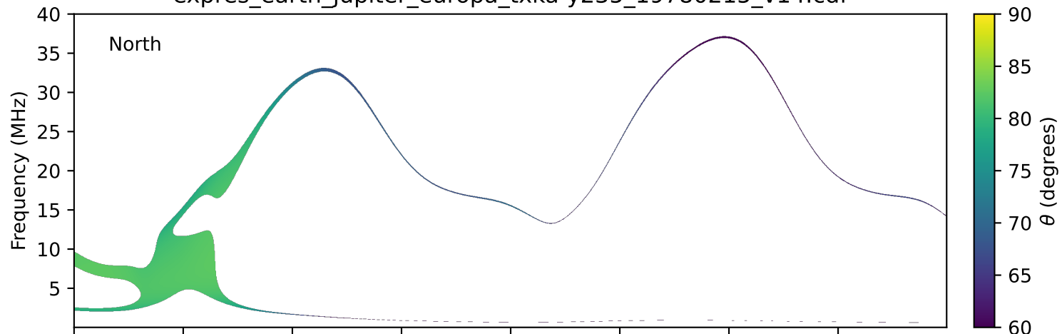
expres_earth_jupiter_europa_txka-y235_19780215_v14.cdf
