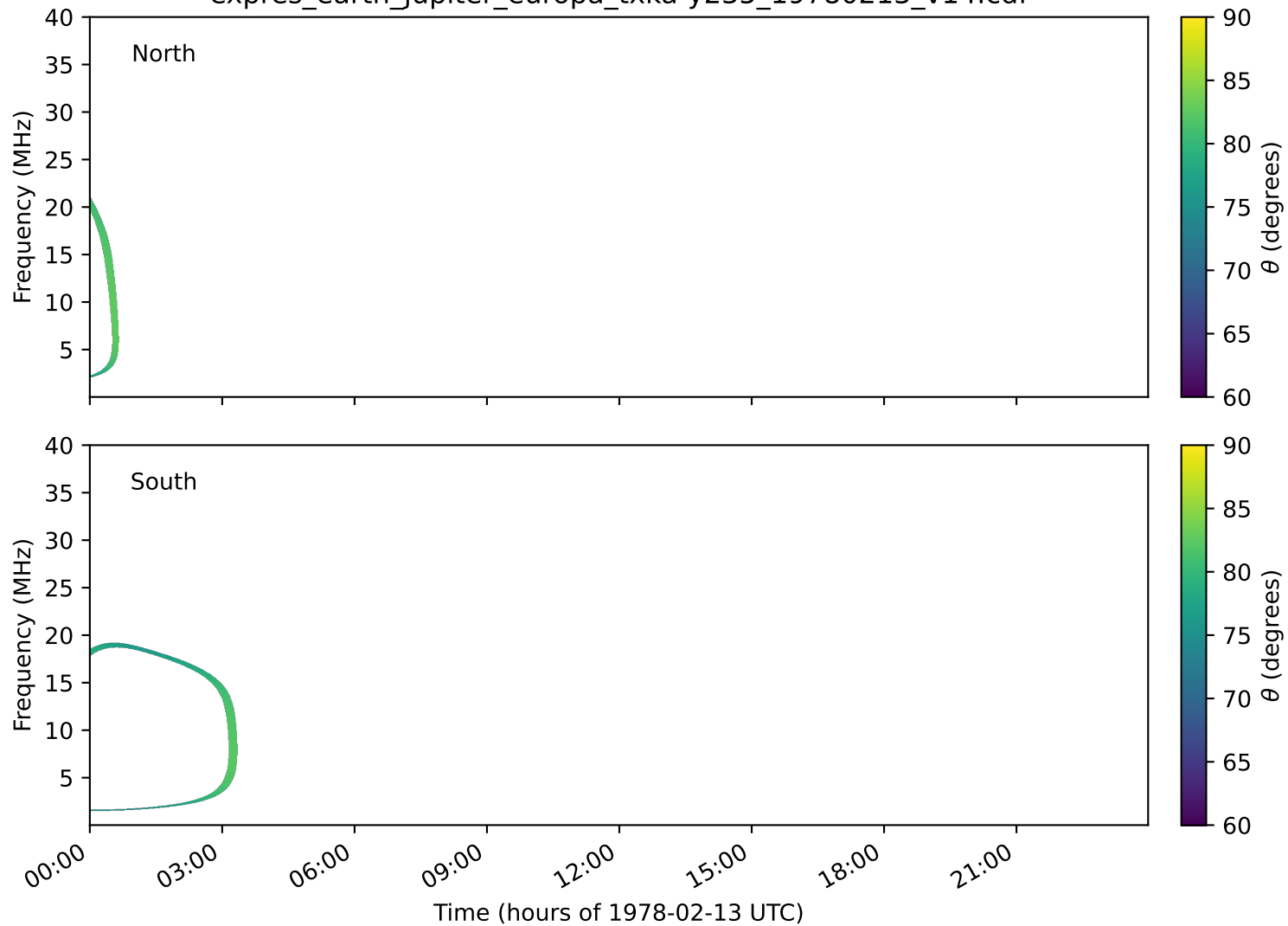
expres_earth_jupiter_europa_txka-y235_19780213_v14.cdf
