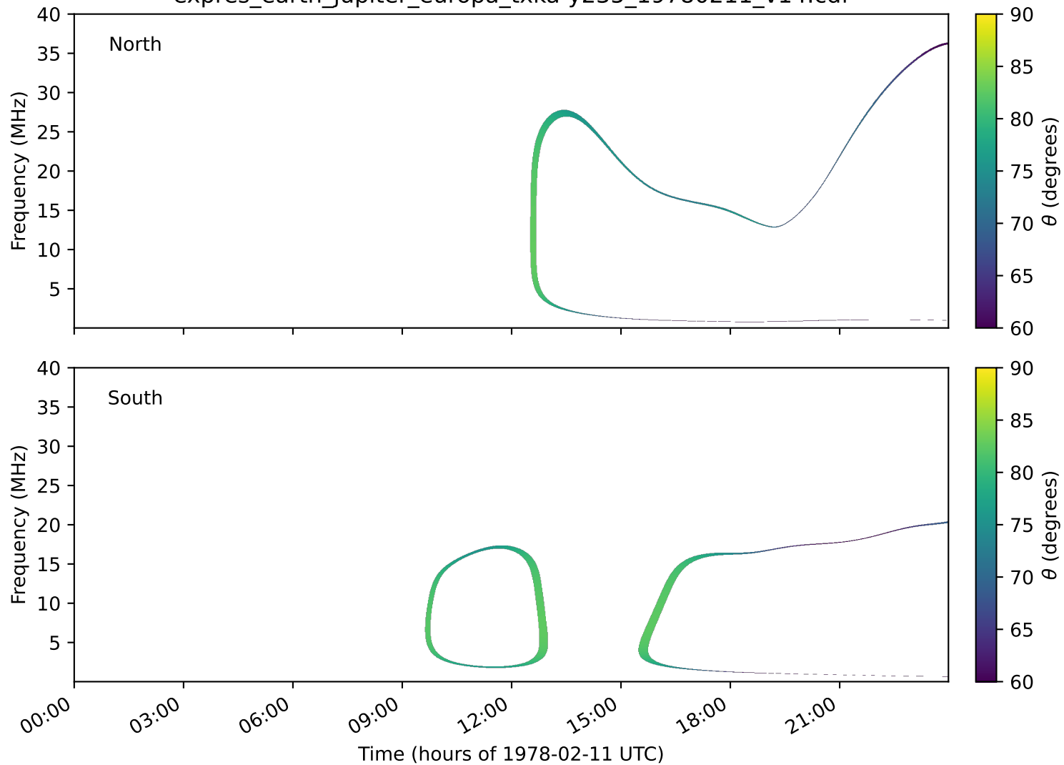
expres_earth_jupiter_europa_txka-y235_19780211_v14.cdf
