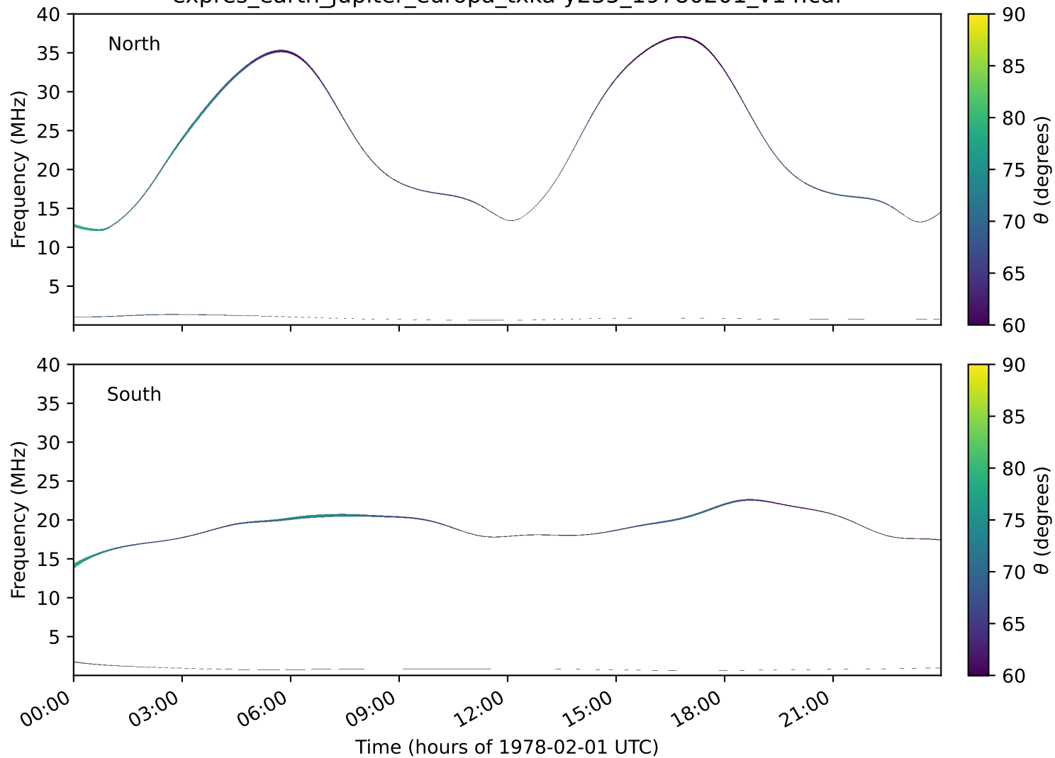
expres_earth_jupiter_europa_txka-y235_19780201_v14.cdf
