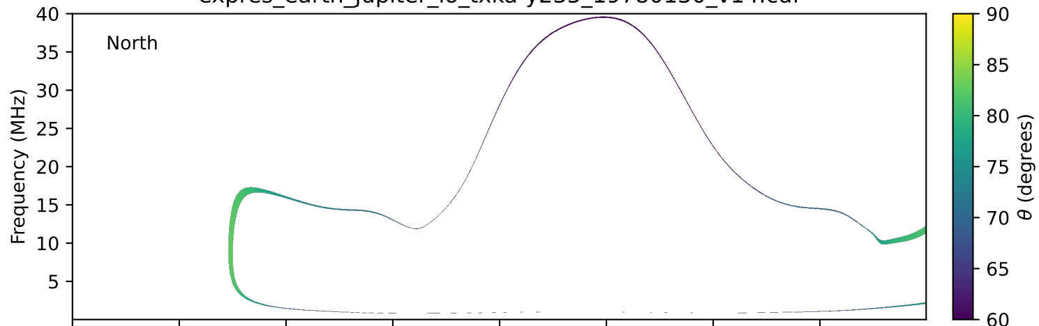
expres_earth_jupiter_io_txka-y235_19780130_v14.cdf
