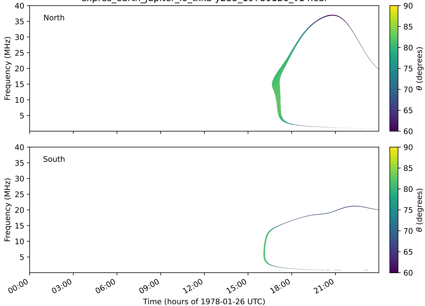
expres_earth_jupiter_io_txka-y235_19780126_v14.cdf
