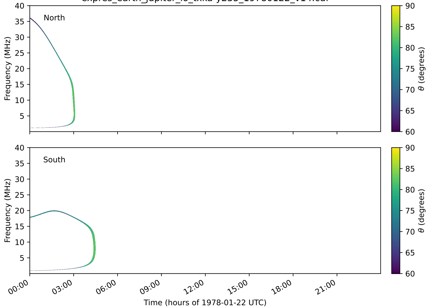
expres_earth_jupiter_io_txka-y235_19780122_v14.cdf
