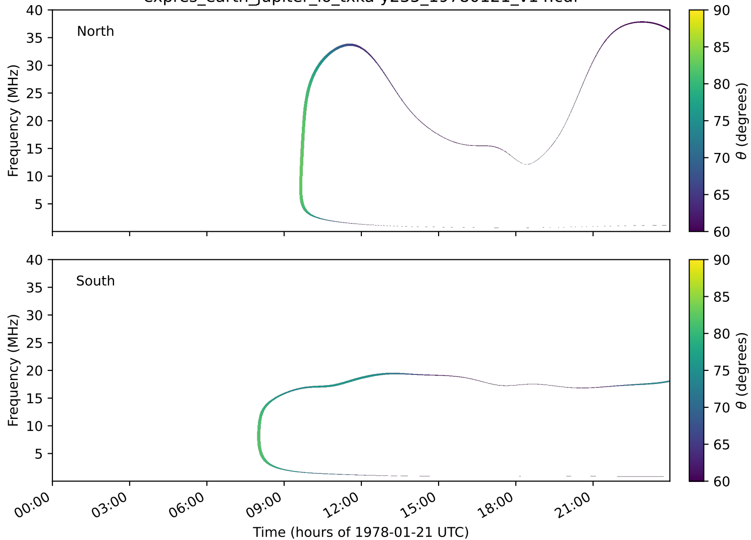
expres_earth_jupiter_io_txka-y235_19780121_v14.cdf
