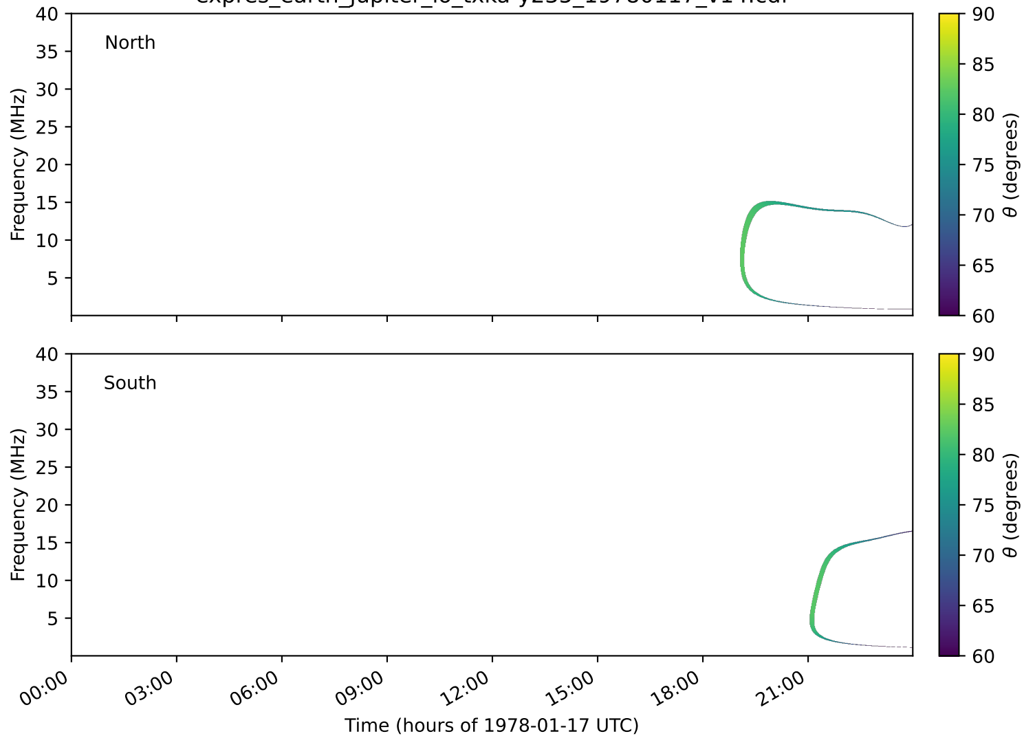
expres_earth_jupiter_io_txka-y235_19780117_v14.cdf
