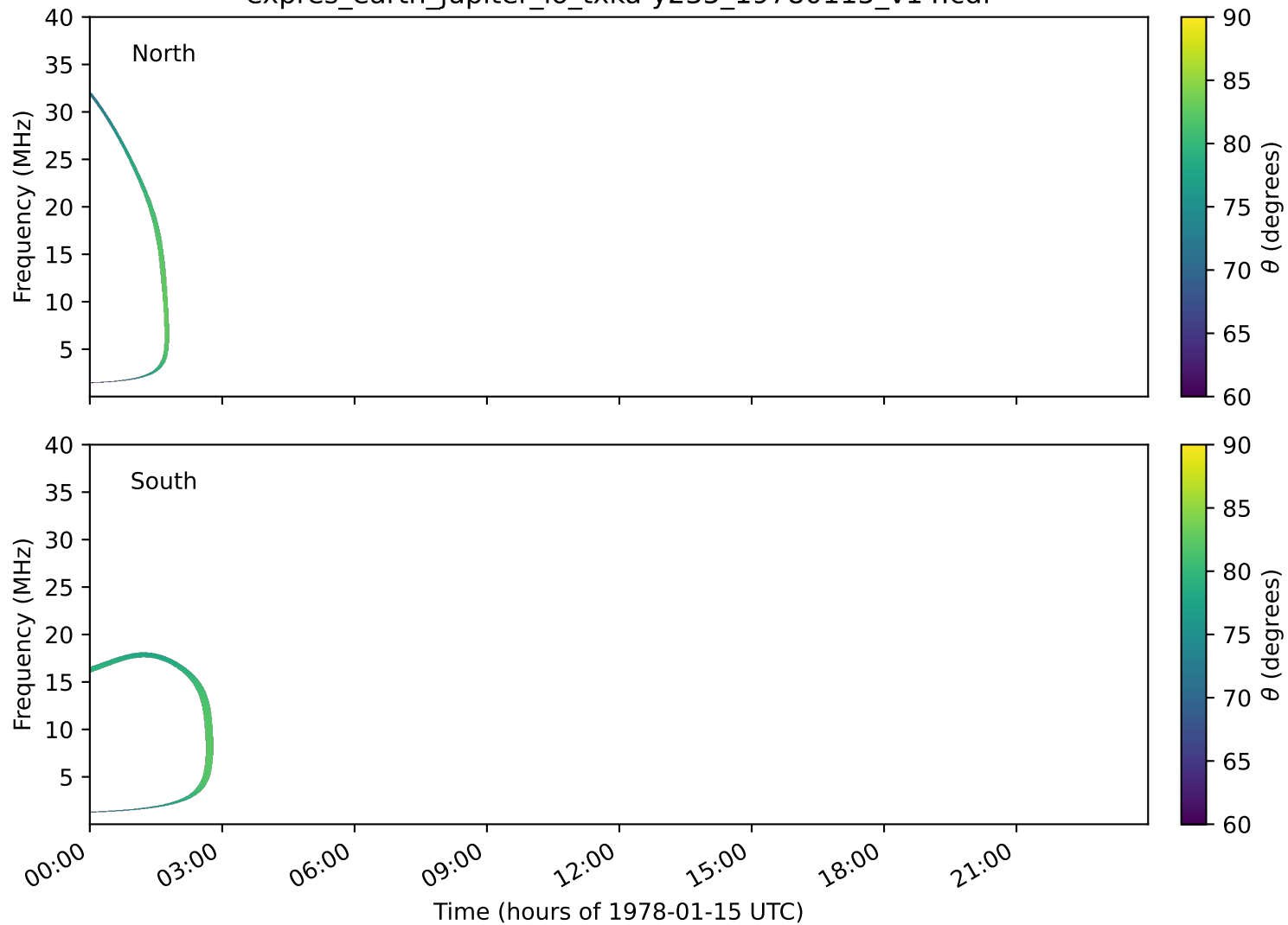
expres_earth_jupiter_io_txka-y235_19780115_v14.cdf
