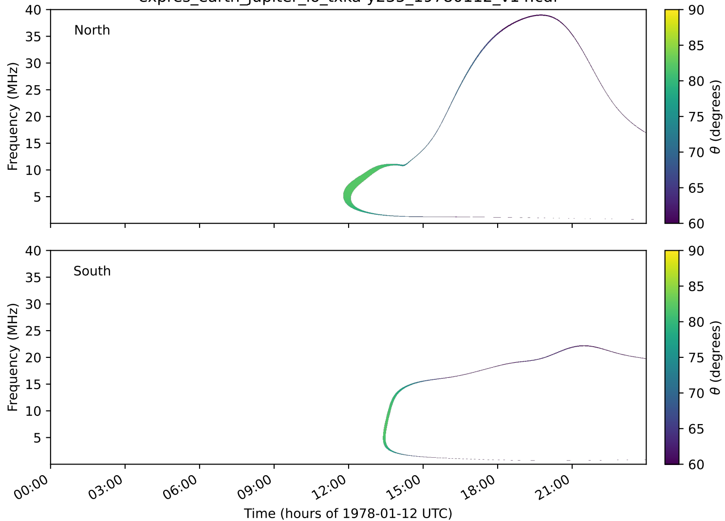
expres_earth_jupiter_io_txka-y235_19780112_v14.cdf
