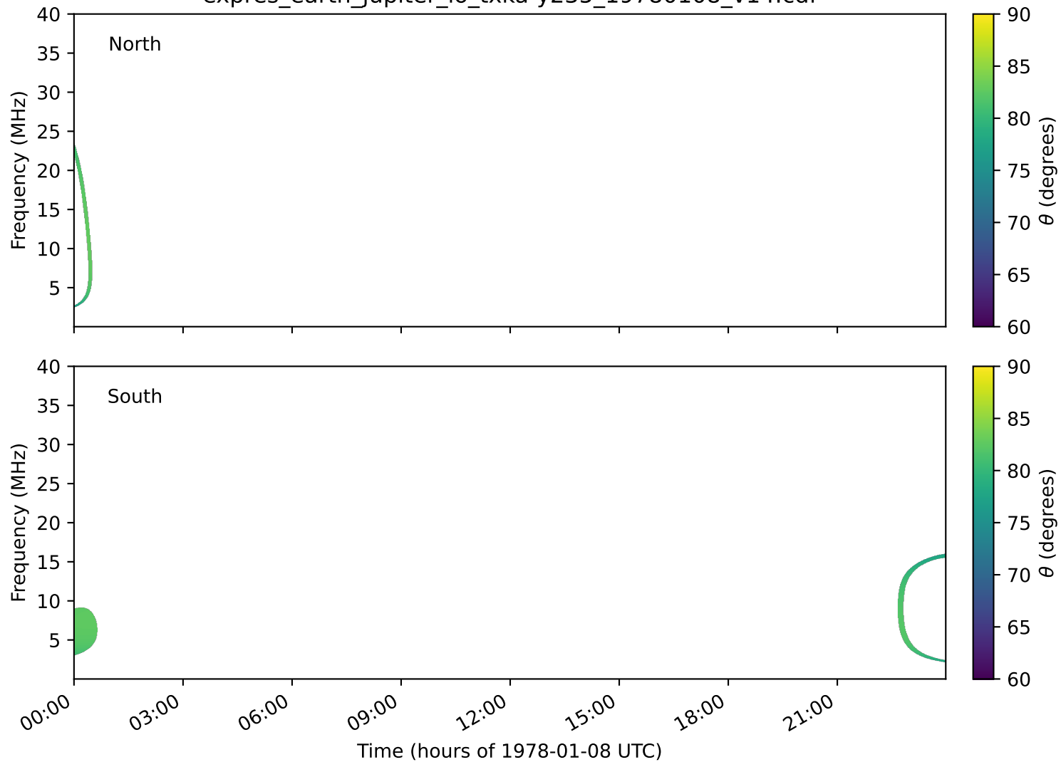
expres_earth_jupiter_io_txka-y235_19780108_v14.cdf
