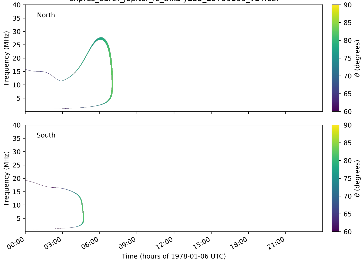
expres_earth_jupiter_io_txka-y235_19780106_v14.cdf
