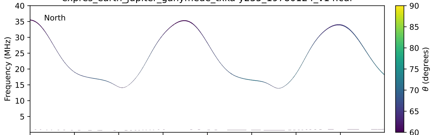
expres_earth_jupiter_ganymede_txka-y235_19780124_v14.cdf
