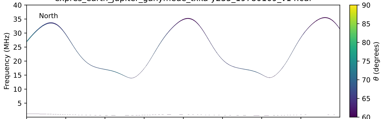
expres_earth_jupiter_ganymede_txka-y235_19780109_v14.cdf
