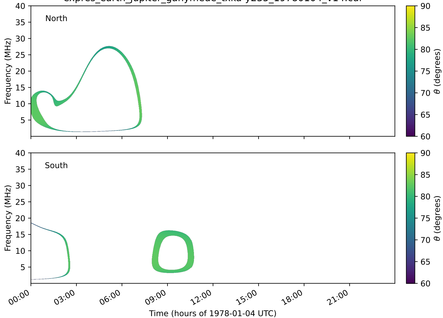
expres_earth_jupiter_ganymede_txka-y235_19780104_v14.cdf
