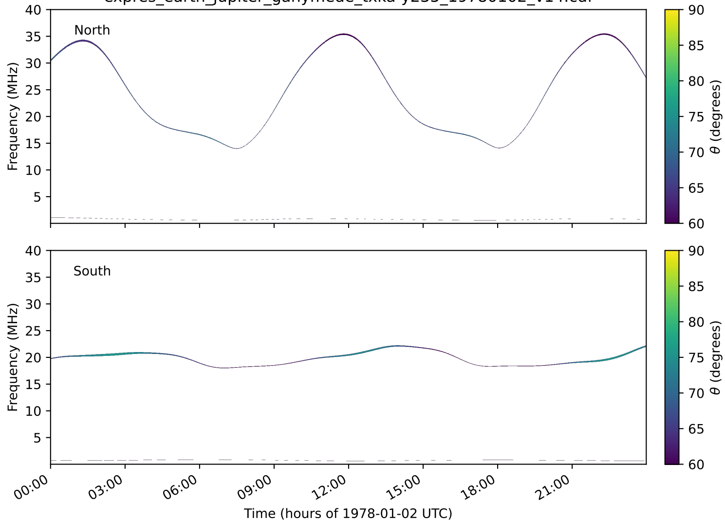
expres_earth_jupiter_ganymede_txka-y235_19780102_v14.cdf
