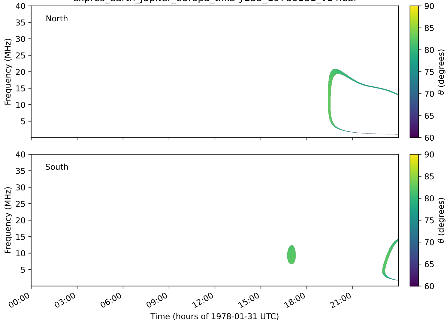
expres_earth_jupiter_europa_txka-y235_19780131_v14.cdf
