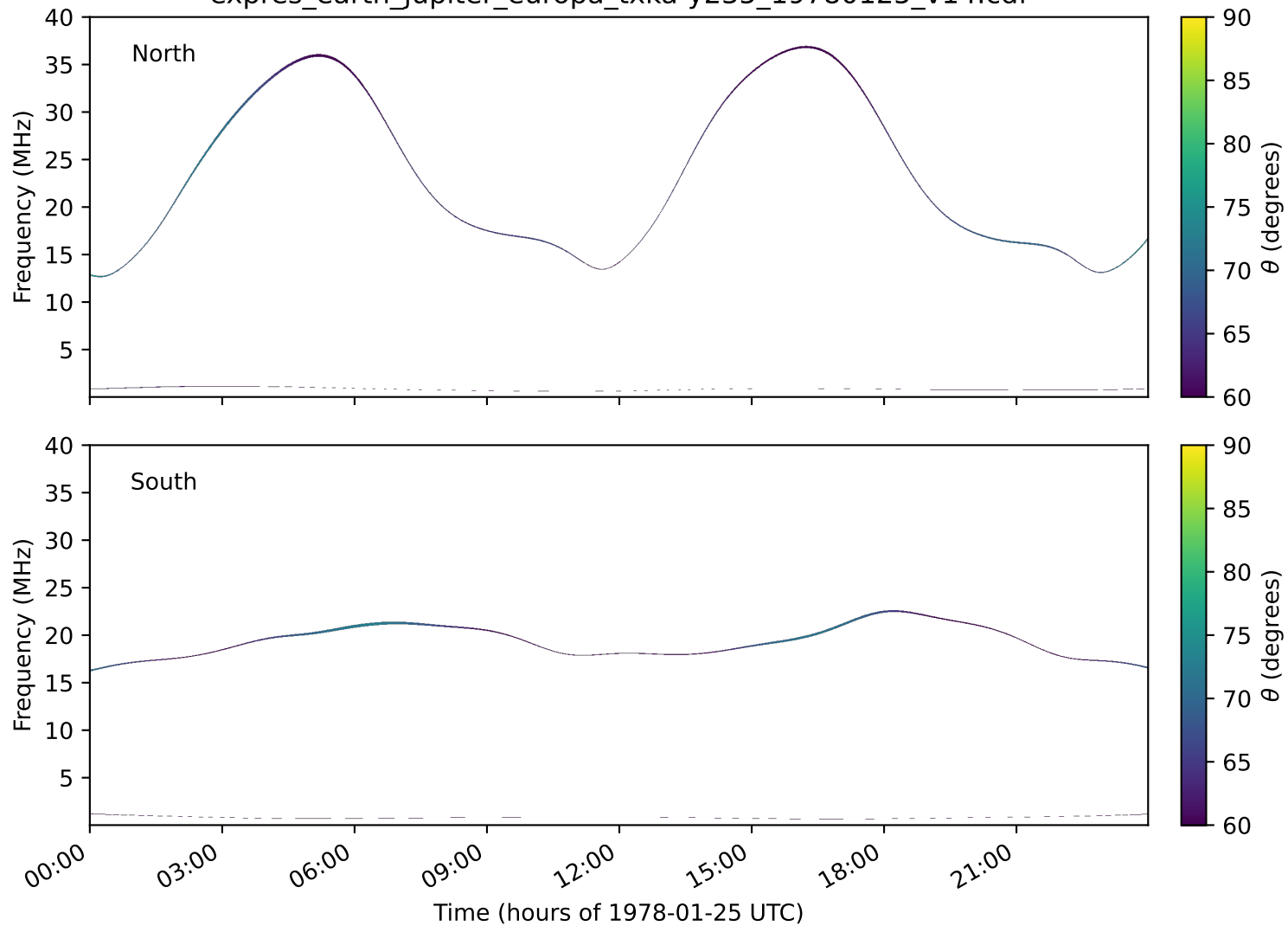
expres_earth_jupiter_europa_txka-y235_19780125_v14.cdf
