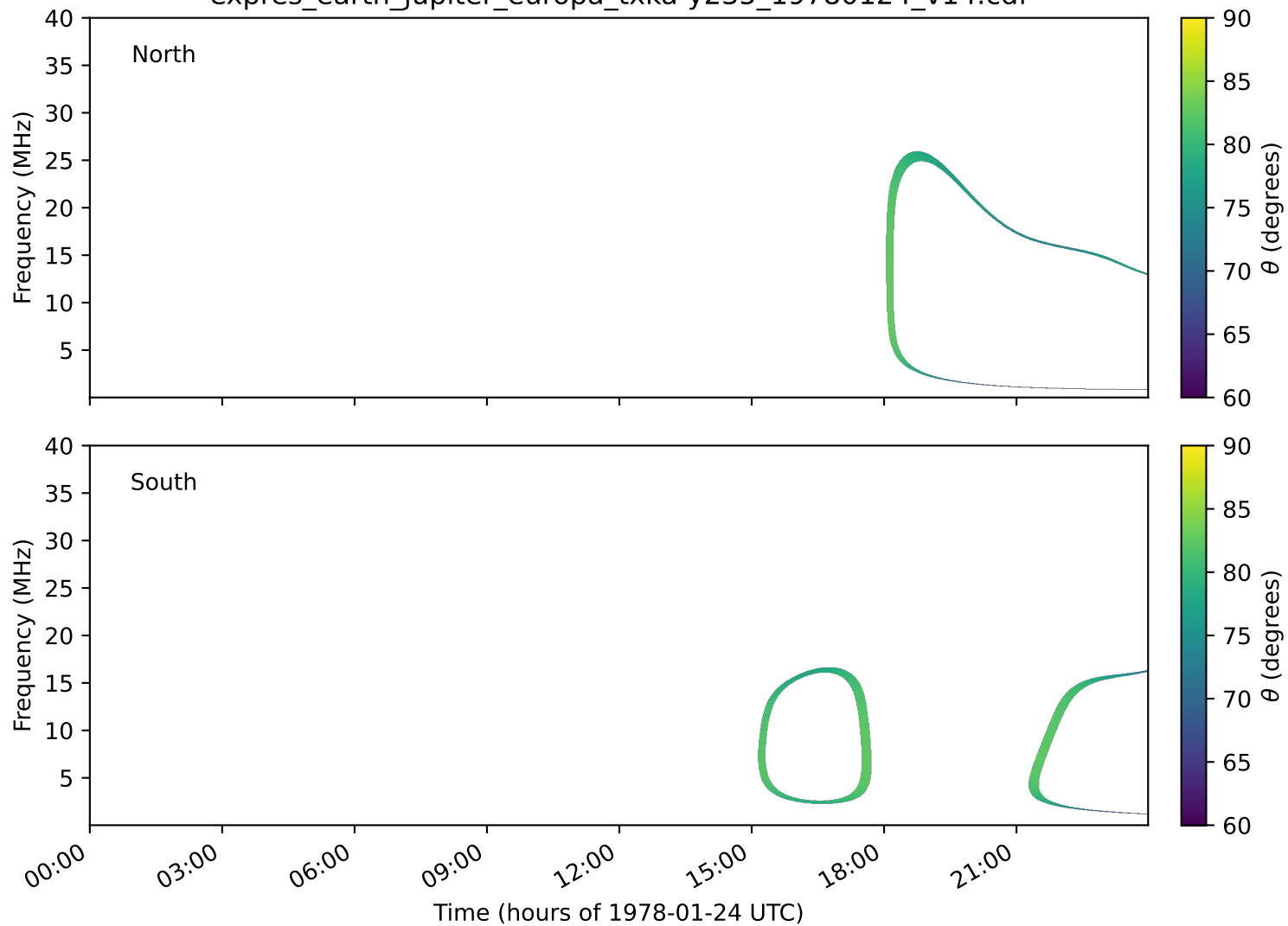
expres_earth_jupiter_europa_txka-y235_19780124_v14.cdf
