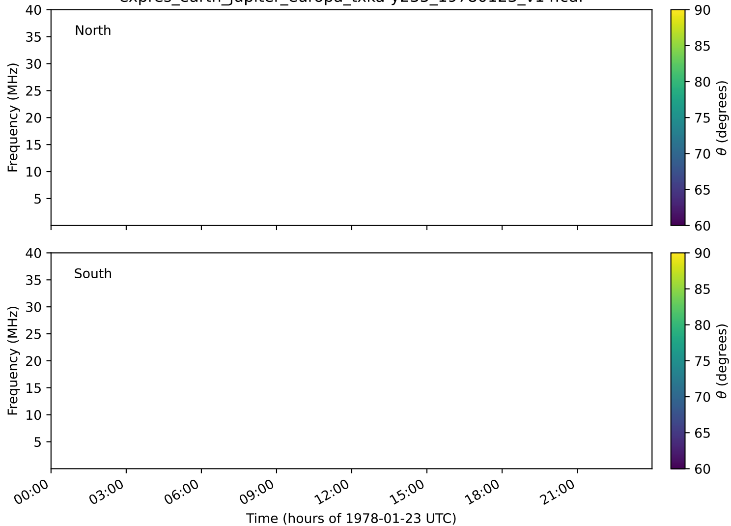
expres_earth_jupiter_europa_txka-y235_19780123_v14.cdf
