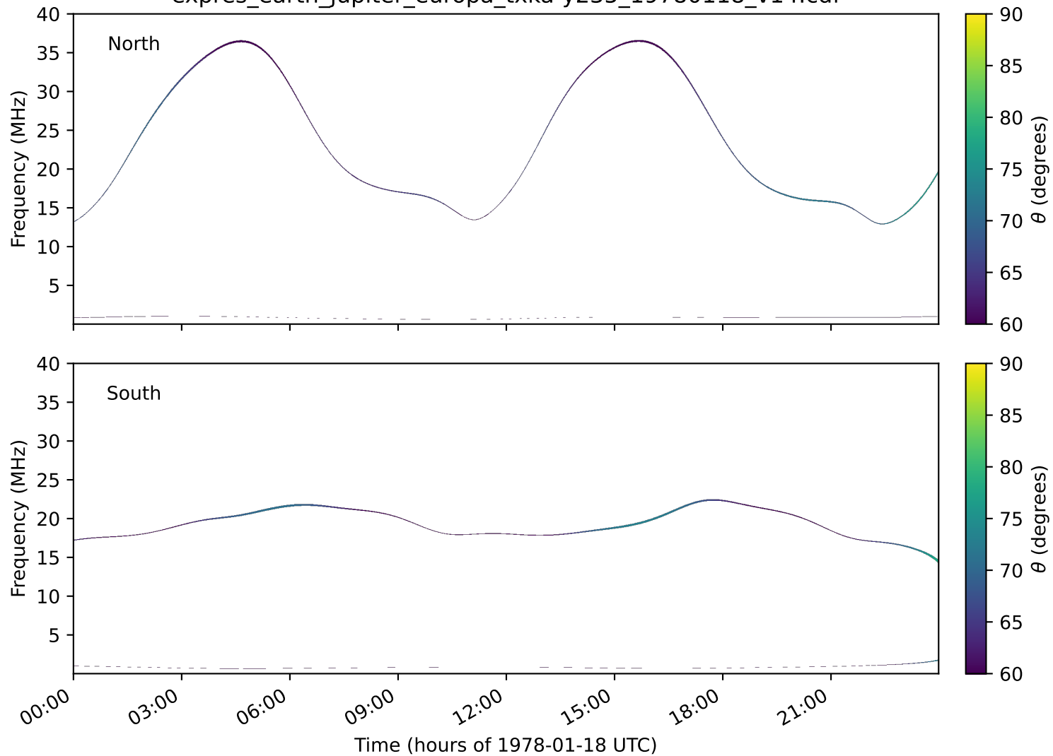
expres_earth_jupiter_europa_txka-y235_19780118_v14.cdf
