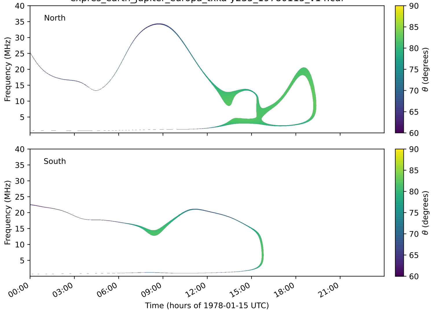
expres_earth_jupiter_europa_txka-y235_19780115_v14.cdf
