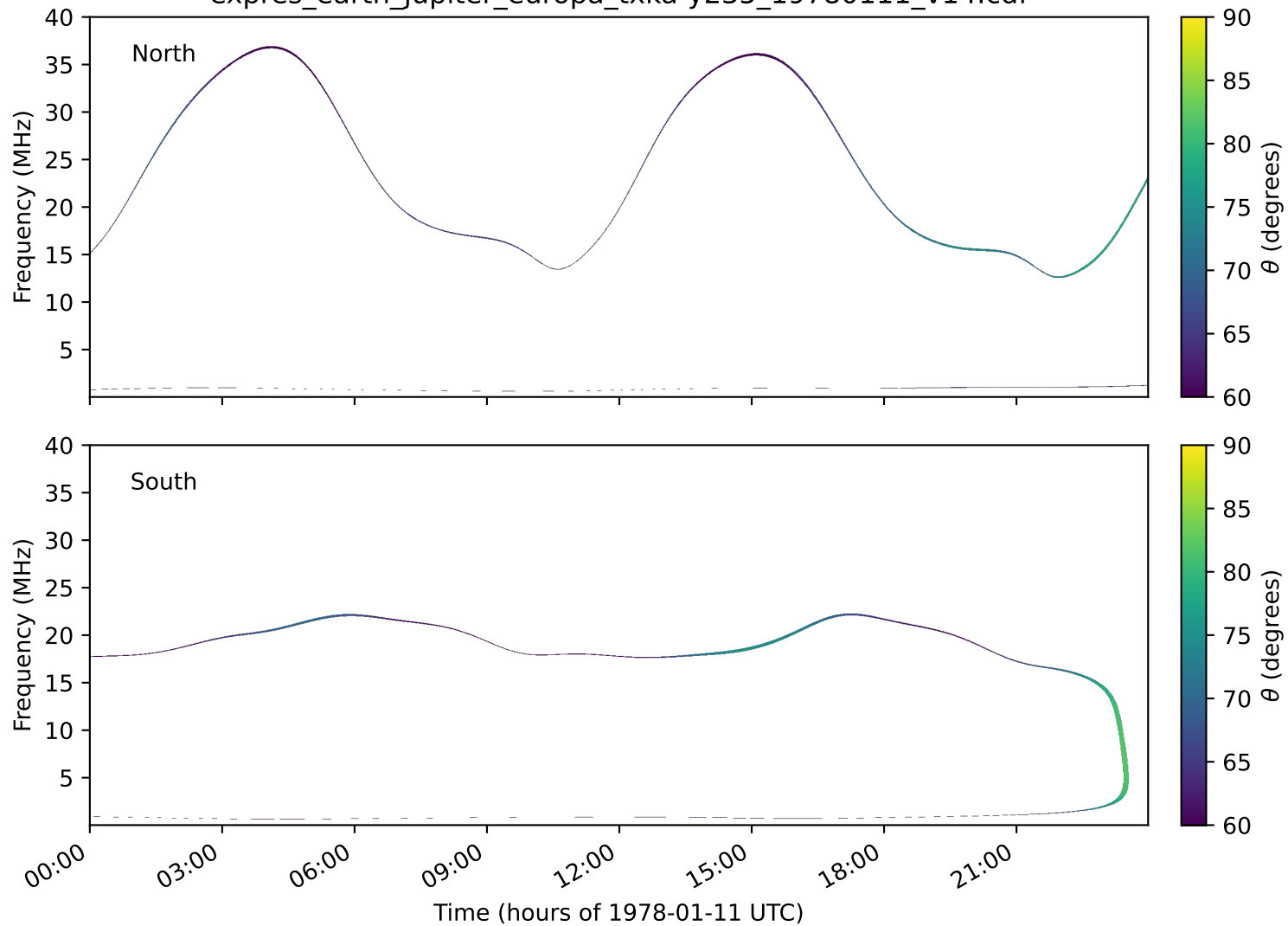
expres_earth_jupiter_europa_txka-y235_19780111_v14.cdf
