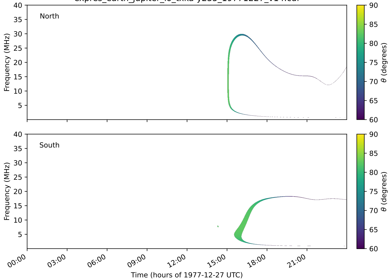
expres_earth_jupiter_io_txka-y235_19771227_v14.cdf
