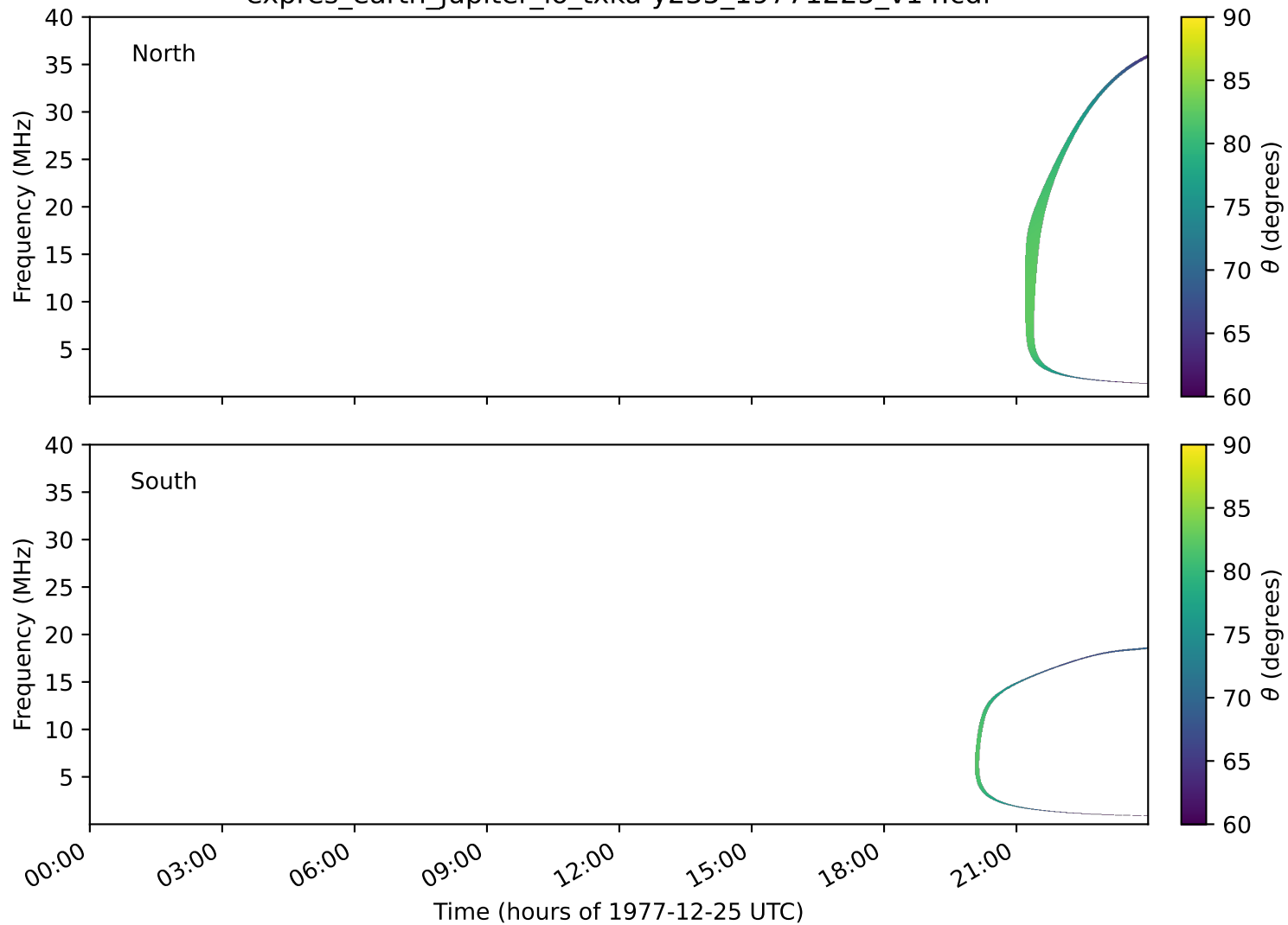
expres_earth_jupiter_io_txka-y235_19771225_v14.cdf
