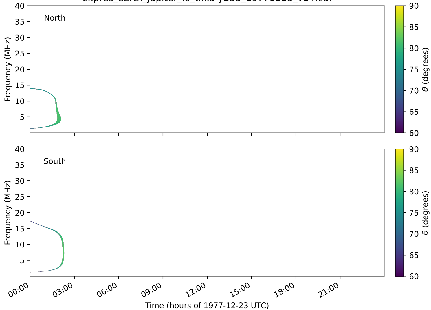
expres_earth_jupiter_io_txka-y235_19771223_v14.cdf
