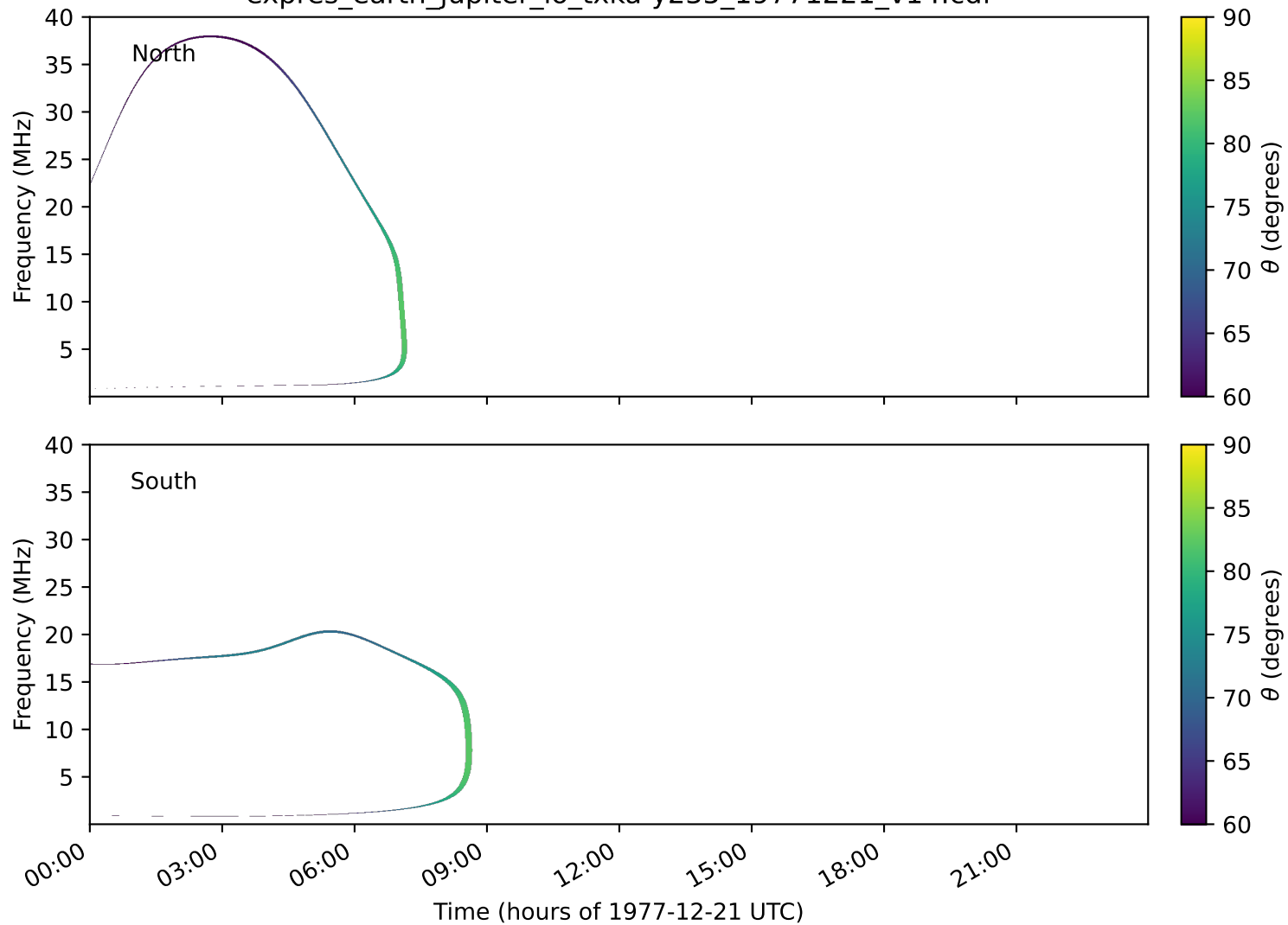
expres_earth_jupiter_io_txka-y235_19771221_v14.cdf
