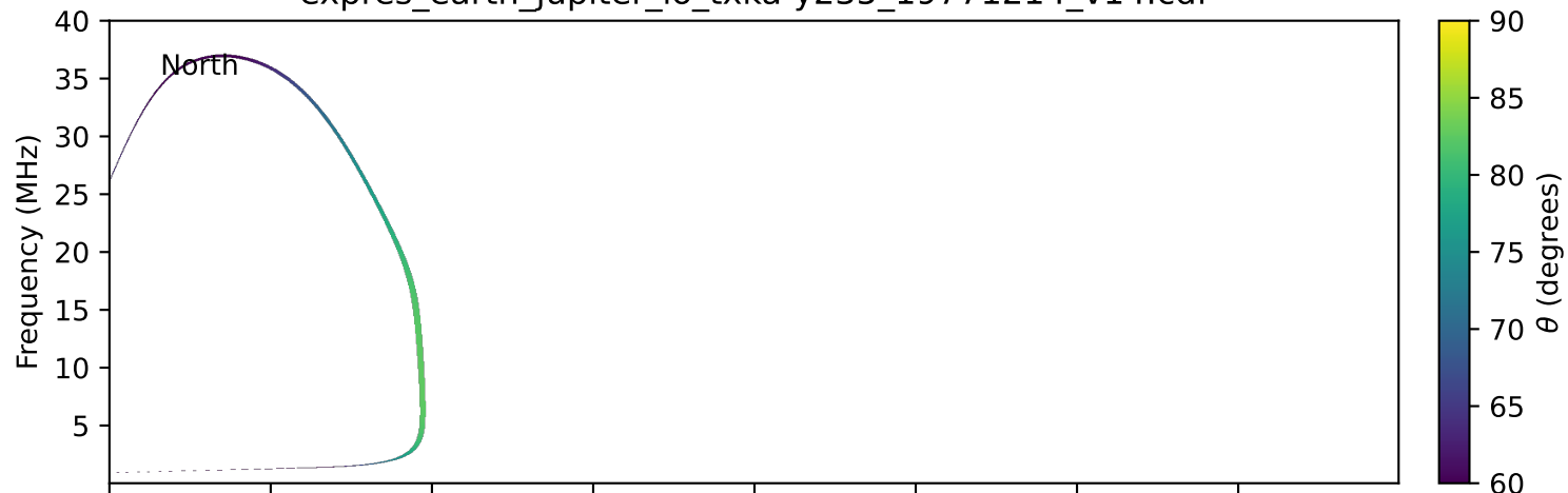
expres_earth_jupiter_io_txka-y235_19771214_v14.cdf
