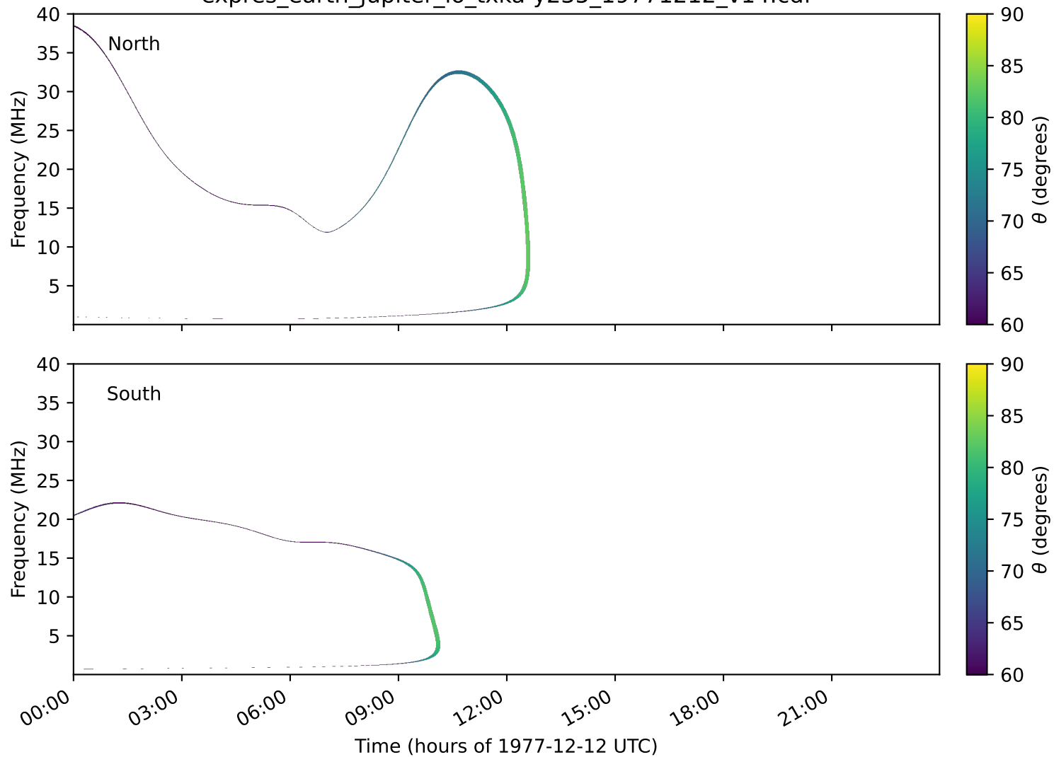
expres_earth_jupiter_io_txka-y235_19771212_v14.cdf
