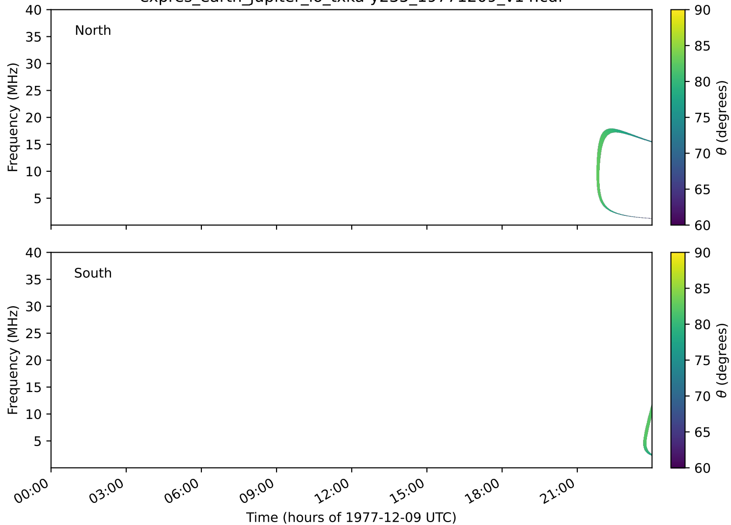
expres_earth_jupiter_io_txka-y235_19771209_v14.cdf
