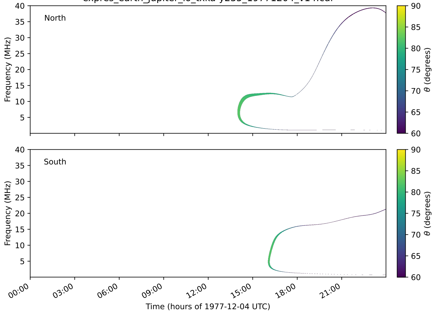
expres_earth_jupiter_io_txka-y235_19771204_v14.cdf
