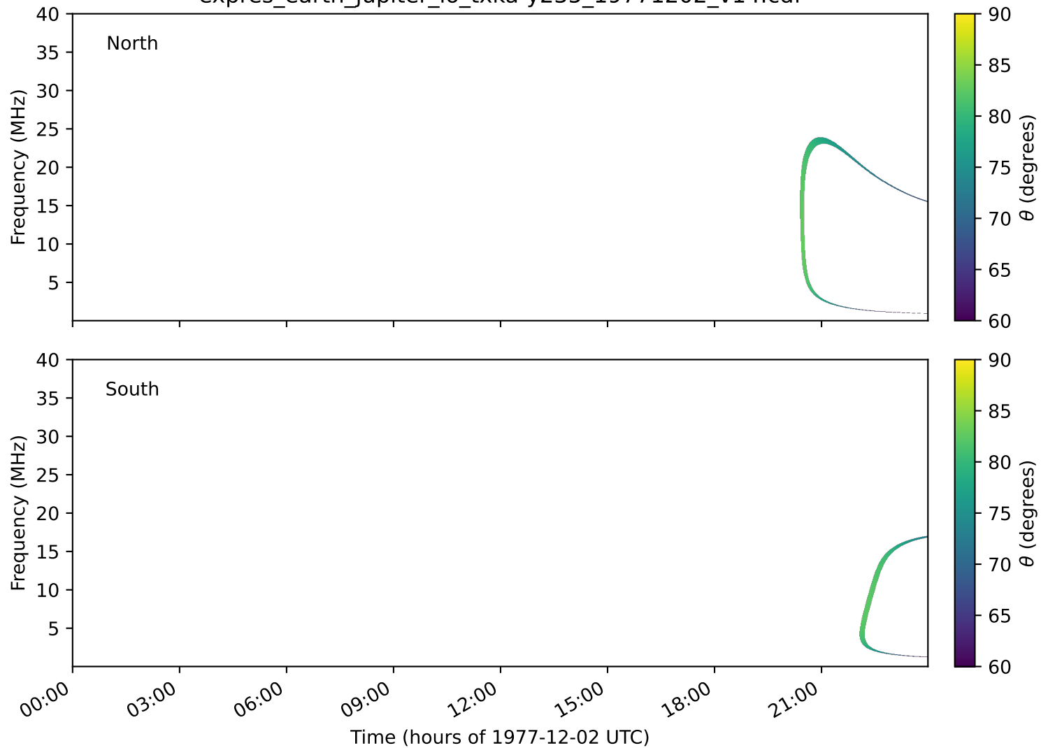
expres_earth_jupiter_io_txka-y235_19771202_v14.cdf
